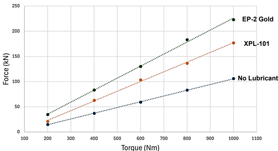
Tensile Force vs Plot of Applied Torque - 1"
